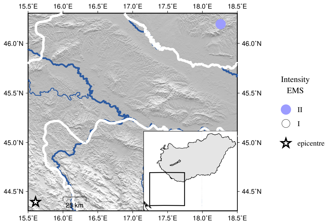
Figure 3.2: EMS intensity distribution for the earthquake of 2025.02.11 17:43 UTC
