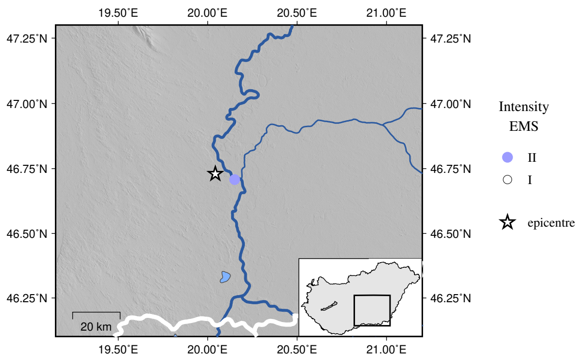
Figure 3.25: EMS intensity distribution for the earthquake of 2025.07.08 14:37 UTC
