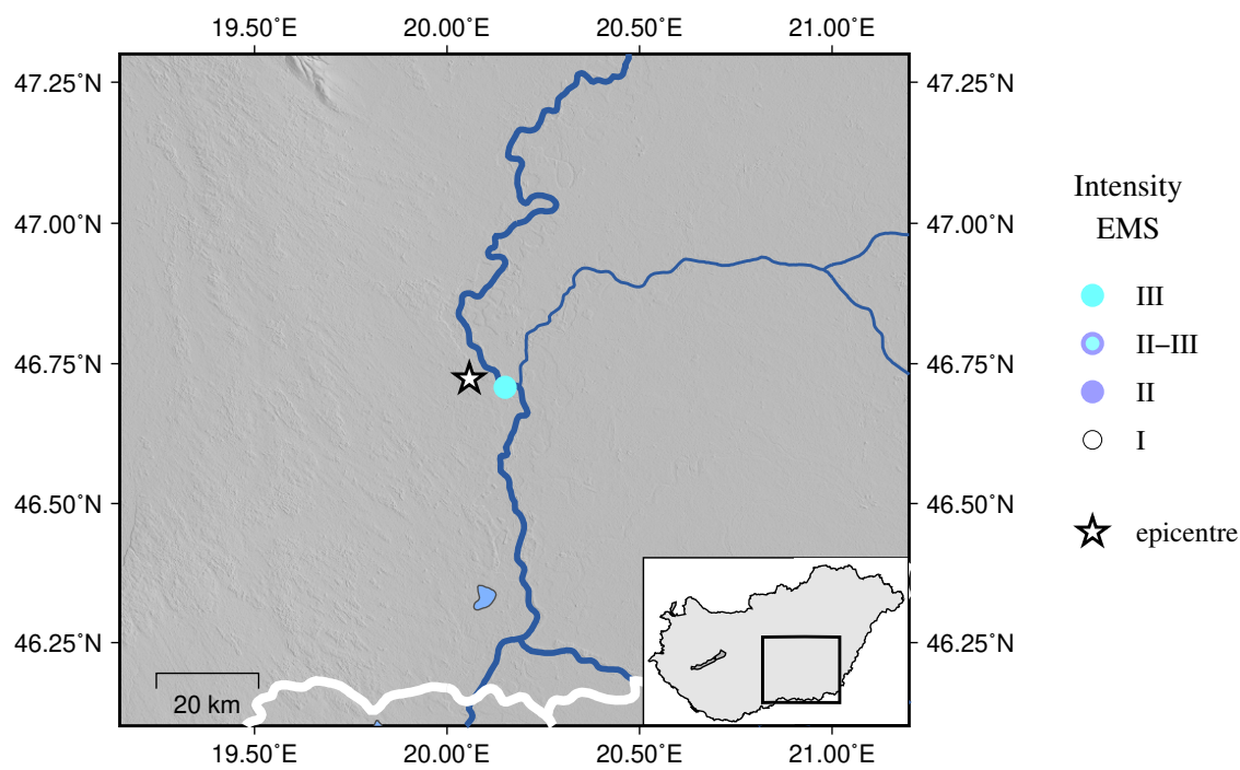
Figure 3.23: EMS intensity distribution for the earthquake of 2025.07.08 07:04 UTC
