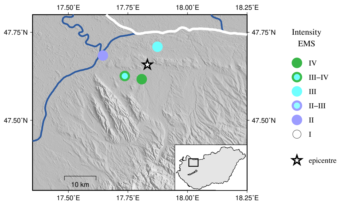
Figure 3.6: EMS intensity distribution for the earthquake of 2025.02.18 11:53 UTC
