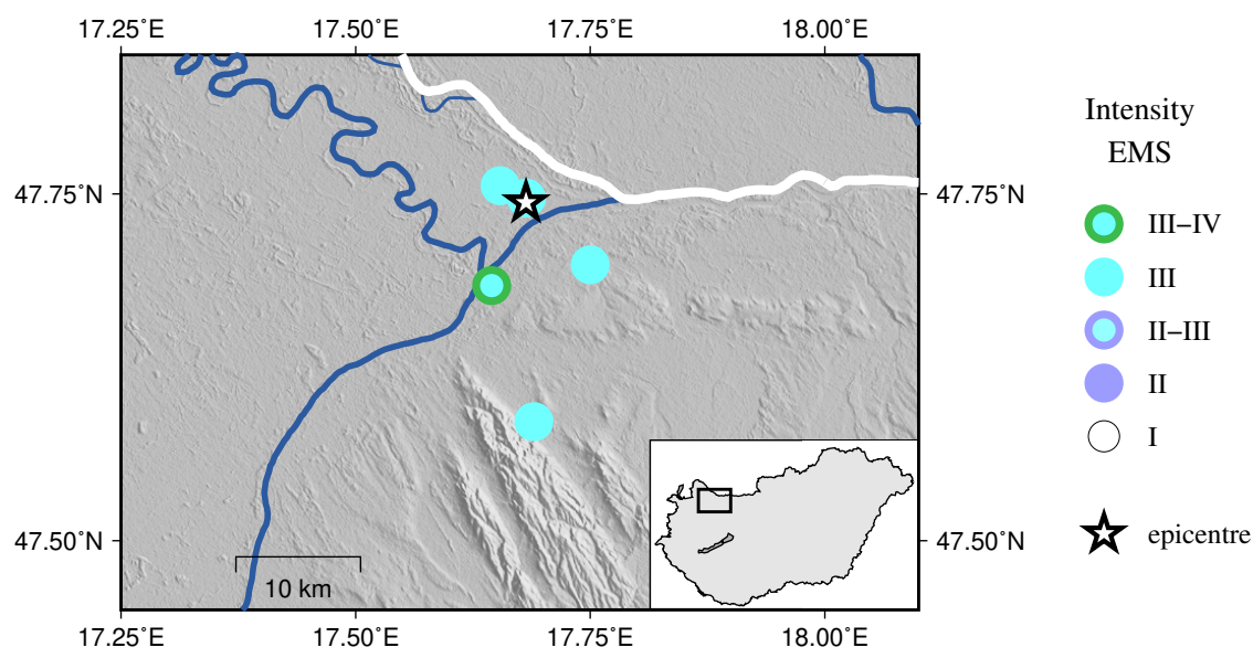
Figure 3.12: EMS intensity distribution for the earthquake of 2025.06.24 18:56 UTC
