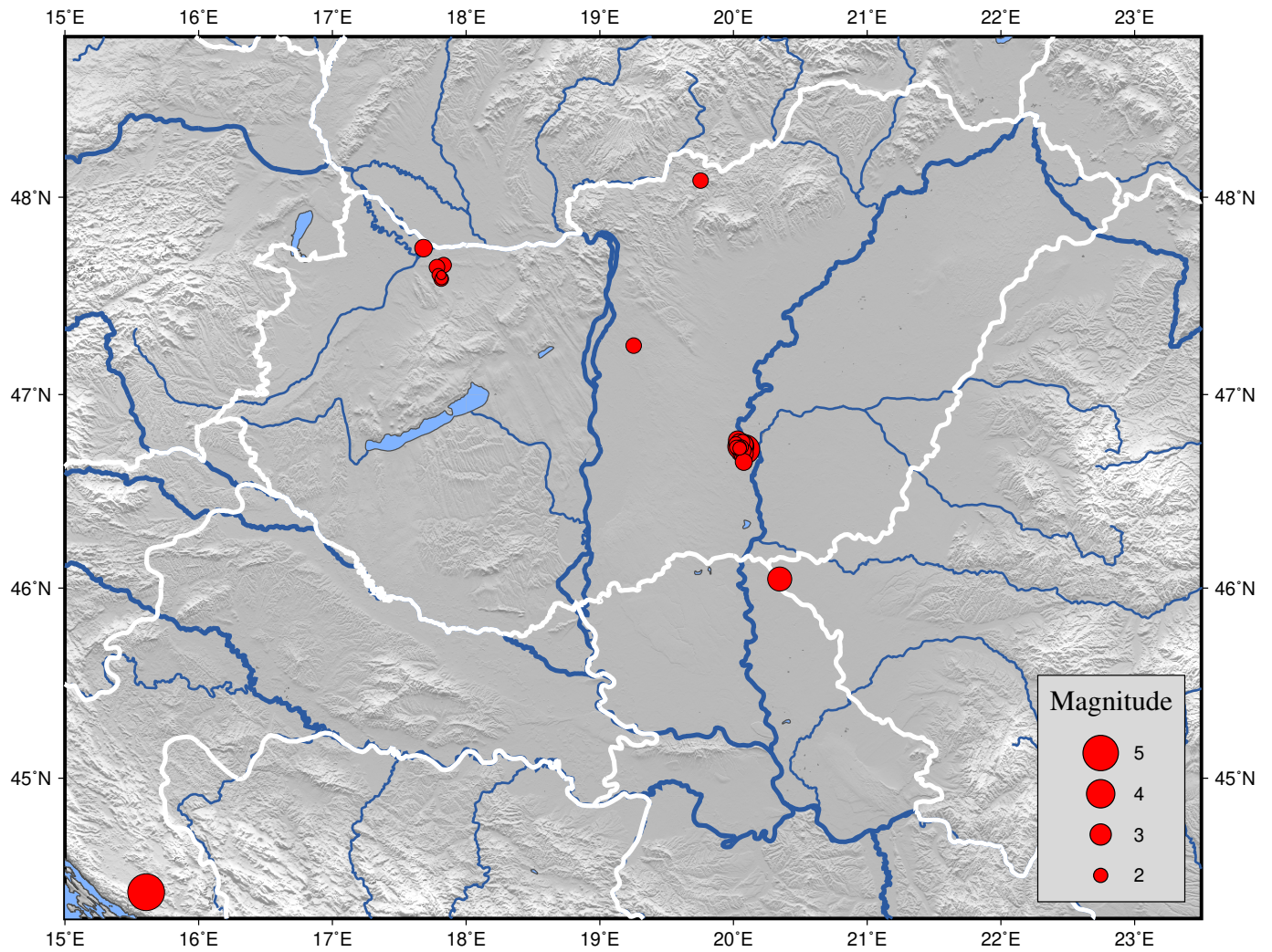
Figure 3.1: The epicenters of the earthquakes felt by the public in Hungary in 2025.
