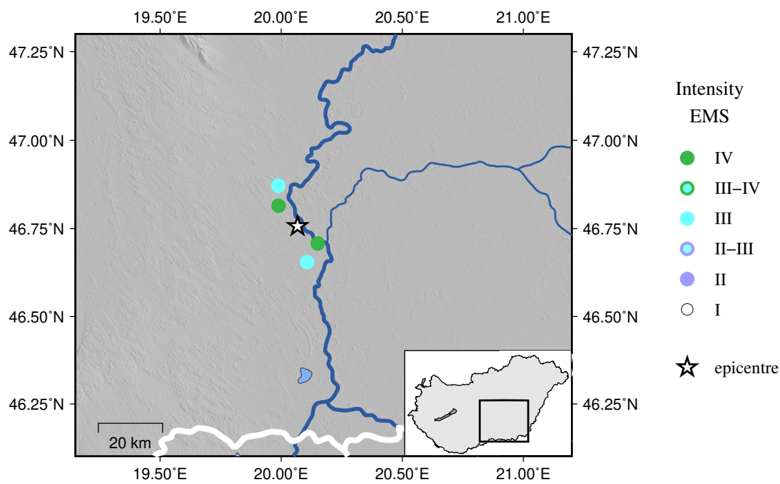
Figure 3.15: EMS intensity distribution for the earthquake of 2025.07.05 19:13 UTC
