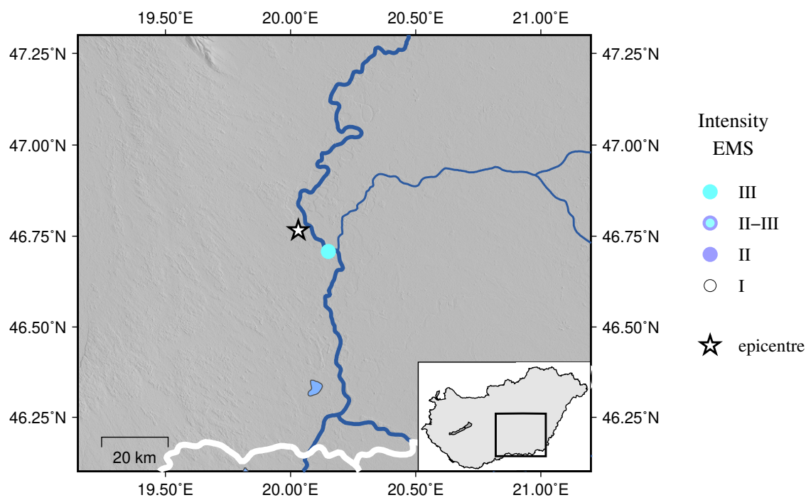
Figure 3.21: EMS intensity distribution for the earthquake of 2025.07.07 07:14 UTC
