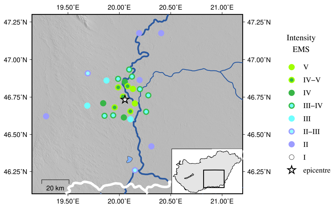
Figure 3.14: EMS intensity distribution for the earthquake of 2025.07.05 18:55 UTC
