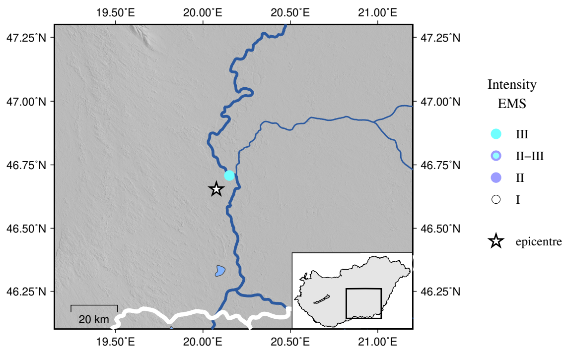
Figure 3.27: EMS intensity distribution for the earthquake of 2025.07.16 13:48 UTC
