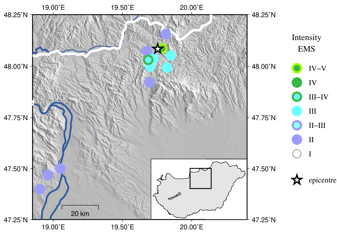
Figure 3.10: EMS intensity distribution for the earthquake of 2025.03.23 19:10 UTC
