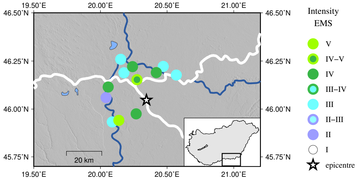
Figure 3.11: EMS intensity distribution for the earthquake of 2025.04.12 05:08 UTC
