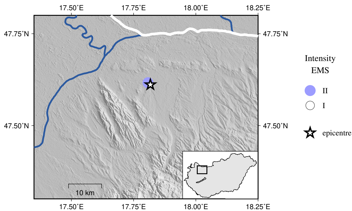
Figure 3.8: EMS intensity distribution for the earthquake of 2025.02.18 20:23 UTC
