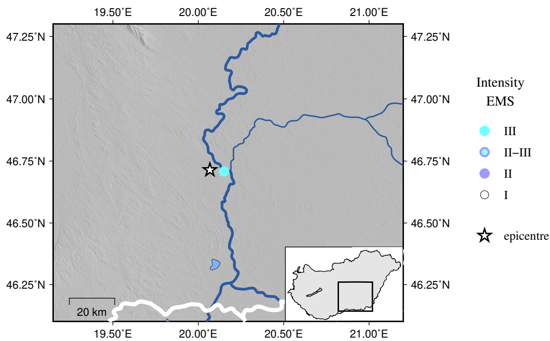
Figure 3.19: EMS intensity distribution for the earthquake of 2025.07.06 02:33 UTC
