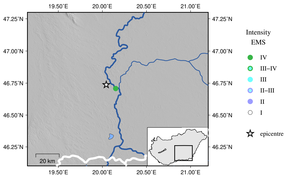
Figure 3.17: EMS intensity distribution for the earthquake of 2025.07.05 23:10 UTC
