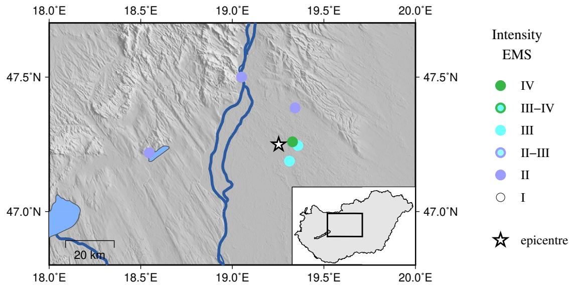
Figure 3.29: EMS intensity distribution for the earthquake of 2025.10.16 17:17 UTC
