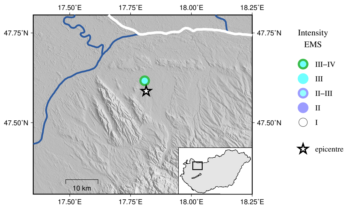
Figure 3.4: EMS intensity distribution for the earthquake of 2025.02.18 06:59 UTC
